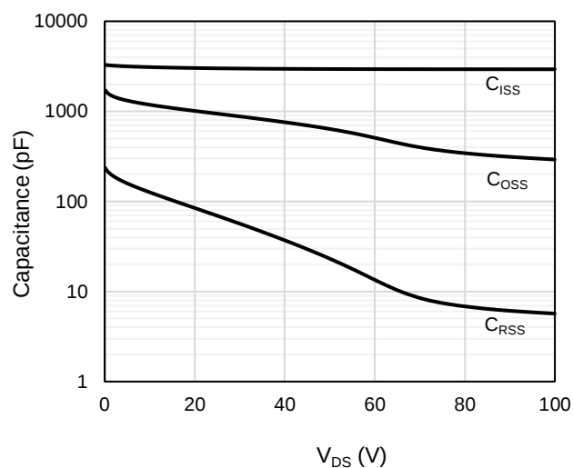
Figure 9: Capacitance Characteristics
